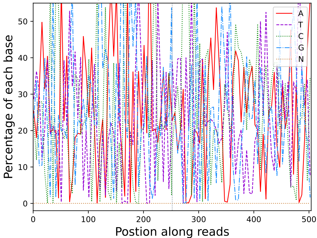
Base percentage along reads (R10522)
